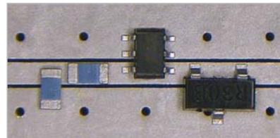
Figure 1 A nominally small SMT part fits well onto the 0.032-in.-wide CPWG 50\ \Omega line structure. The 0603 resistors and capacitors and a small gallium-arsenide FET-amplifier SC-70 IC also fit well.
