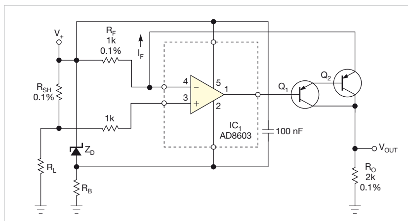
Figure 1 The circuit senses the current flowing through load resistor R L at the high side and transfers it directly to the low side by means of feedback current I F , which has 500 \mu\text{A} at full-scale.
