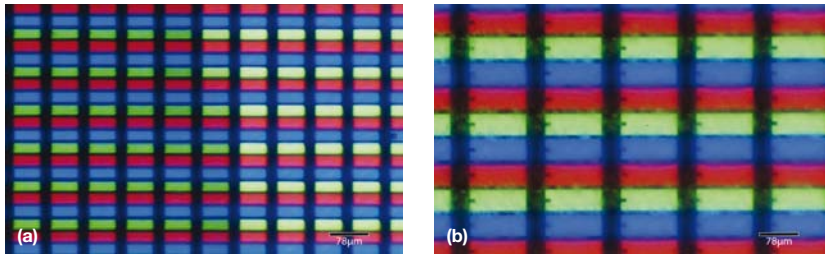
Figure 3 The high-resolution Retina display (a) squeezes four times the pixels into the same screen real estate as its conventional LCD predecessor (b).
